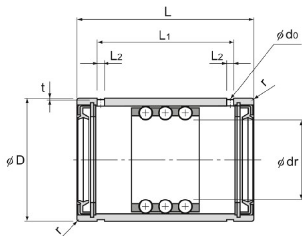
Model ST...UU (For light load)
