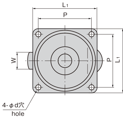
[K-100AF]
