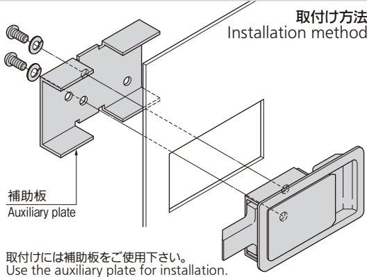
[C-1201-2 右用] Right-hand use
