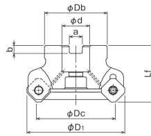
Type1 油穴付き With coolant hole
