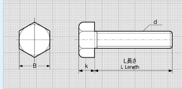
外形寸法図 Dimensional Outline Drawing
