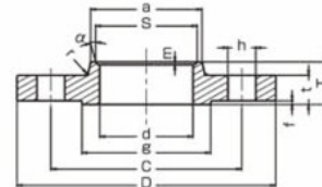
SORF (A type) Slip on Flange RF
