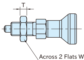
NDXN-W-ASUS NDXN-AW-ASUS (Double-Nut)
