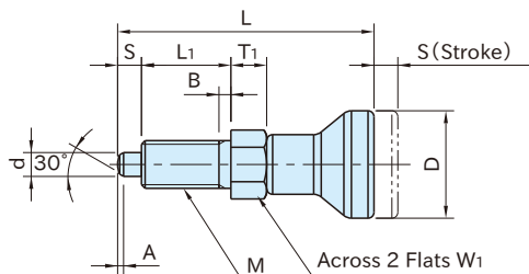
NDXN-ASUS NDXN-A-ASUS (Single-Nut)
