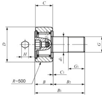
CF...BR Stud dia d_1 3-10mm
