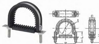
Anti-vibration stainless steel U-band with plate
