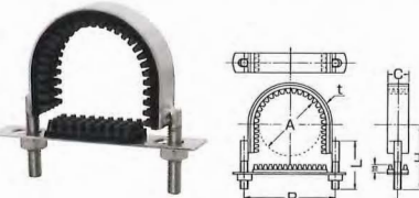
Anti-vibration stainless steel U-band with plate
