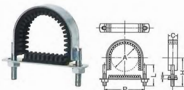
Anti-vibration U-band with plate
