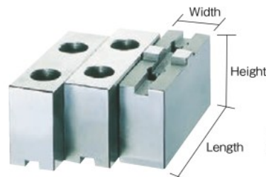
SJ Type (3 pieces 1 set)
