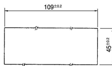
Panel mounting hole
